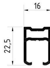
AL-IS.2 U-Führung Art.-Nr. 3003021FF
