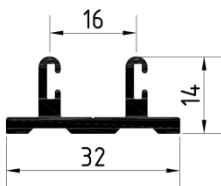
AL-IS.2 U-Bodenschiene ST Art.-Nr. 3003026FF
