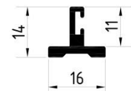
AL-IS.2 Bodenschiene ST Art.-Nr. 3003025FF
