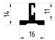
AL-IS.2 T-Bodenschiene ST Art.-Nr. 3003025FF
