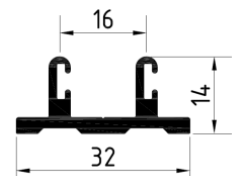
AL-IS.2 U-Bodenschiene ST Art.-Nr. 3003026FF
