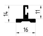
AL-IS.2 T-Bodenschiene ST Art.-Nr. 3003025FF
