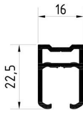
AL-IS.2 U-Führung Art.-Nr. 3003021FF
