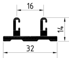
AL-IS.2 U-Bodenschiene ST Art.-Nr. 3003026FF
